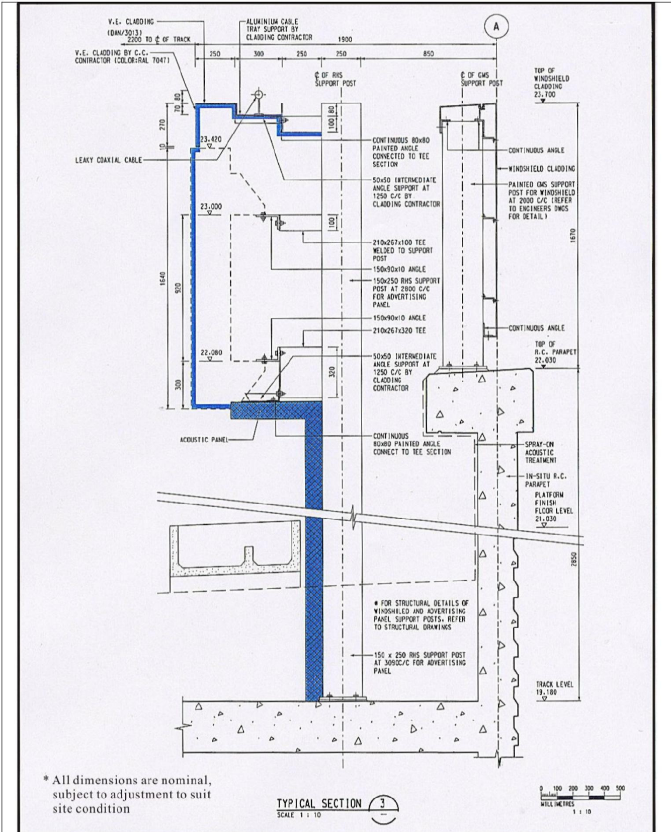
Figure 5 – Trackside Panels and Windshields at the Yuen Long Station [Uptrack (track from Kowloon to Tuen Mun)]
